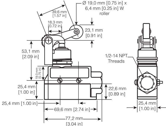
Figure 5. Roller lever, adjustable, side mount with boot seal
